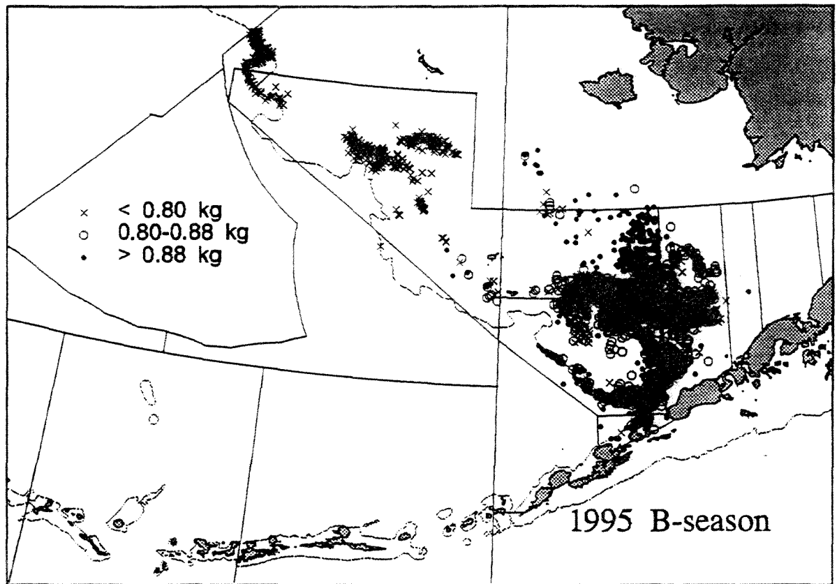
Fig. 2--Trawl locations in the 1995 pollock B-fishery. Symbols indicate mean pollock weight in the trawl: < 0.80 kg (x); 0.80-0.88 kg (o); and > 0.88 kg (•). (Source: M. Sigler Alaska Fisheries Science Center, Auke Bay Laboratory, 11305 Glacier Hwy, Juneau, Alaska, 99801).
