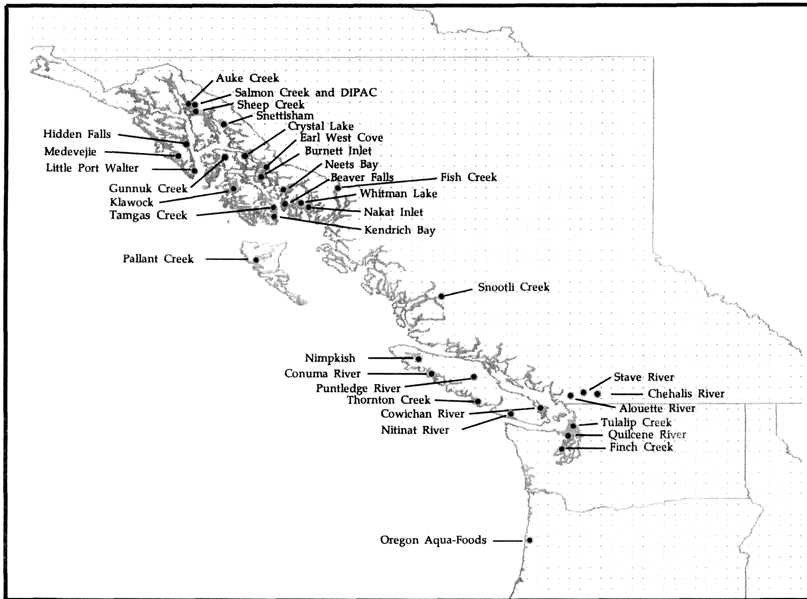
Fig. 5--Location of Southeast Alaska, British Columbia, and Washington hatcheries releasing CWT chum salmon from 1980 to 1993. (Source: Pacific States Marine Fisheries Commission).
