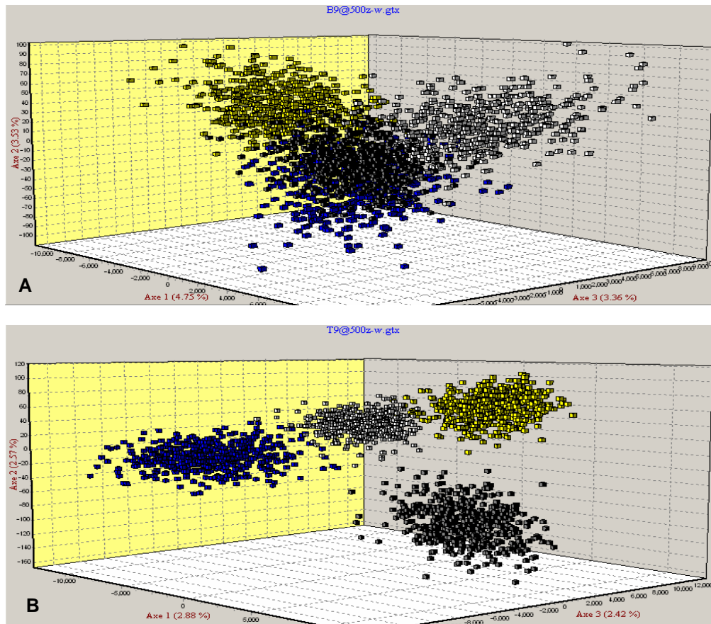
Fig. 1. Factorial correspondence analysis using data of 500 samples per Chinook life history type, simulated using WHICHLOCI (Banks et al. 2003) and analyzed using GENETIX (Belkhir et al. 2002). Square plots represent individual salmon samples colored in accord with their life-history type and positioned on the graph in relation to their genetic relationship. This is approximated from either: A. nine loci from the bottom of the rank depicted in Table 1 or B. nine loci from the top of this same rank. Tighter clustering of life-history types and zero overlap in B demonstrates the power gained through using loci with greater information content.
