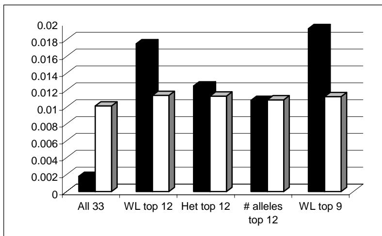
Fig. 2. Genetic stock Identification results using the population based GMA method of Kalinowski (2003). One thousand simulated fishery samples had N = 500 . For fair comparison with individual based methods, relative component estimates were set with the two spring life history types and late fall each at a frequency equivalent to just one fish in the 500 fishery sample (0.002), setting the remainder for the components made up almost equal proportions of fall (0.442) and winter (0.522). Bars shown in black depict the absolute sum of the differences between observed and expected frequencies across all life history types and bars shown in white depict average standard deviation. Paired columns are displayed according to alternate loci combinations used: From left to right, all 33 loci together, 12 loci that ranked highest using WHICHLOCI, 12 loci with highest heterozygosities, 12 loci with the greatest number of alleles and lastly 9 loci that ranked highest using WHICHLOCI.
