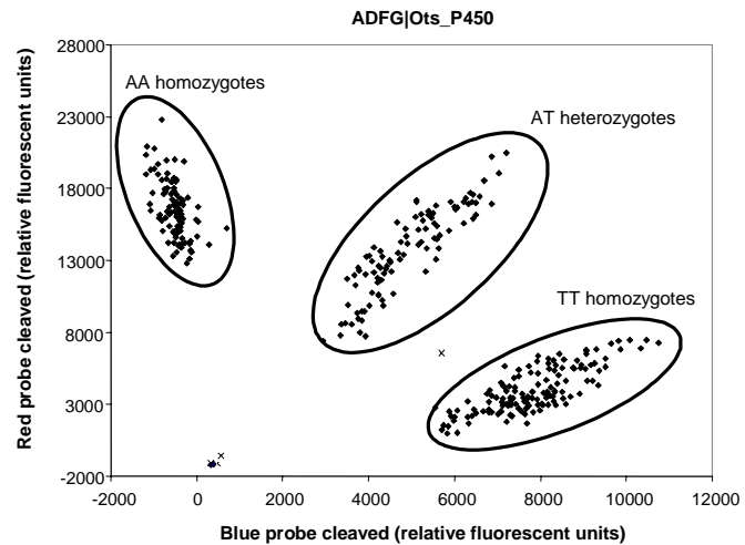
Fig. 2. Analysis of data produced by genotyping 380 fish using the 5'-nuclease reaction. Sequence Detection Software V. 2.0 (Applied Biosystems Inc.) was used to generate the chart below in which the two axes represent the amounts of signal from each of the allele-specific probes. Each dot on the chart below represents an individual fish, whose genotype is determined by where its dot falls on the axis. The circles indicate clusters of a single genotype each. Mitochondrial DNA assays produce two clusters while nuclear DNA assays (such as the example below) produce three clusters. The "x"s represent unreadable samples (air-bubbles, failed PCRs etc.) and the dots in the bottom left corner are the negative controls (no template DNA added).
