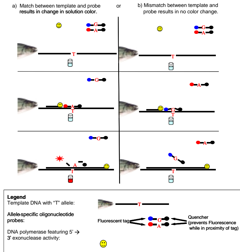
Fig. 1. Genotyping via the 5'-nuclease reaction involves adding allele-specific fluorescent oligonucleotide probes to a typical polymerase chain reaction. During the reaction the probes anneal to the template DNA either (1a) perfectly or (1b) imperfectly. In the former case, the probe is cleaved causing fluorescence. In the latter case, the probe is simply knocked free and no color change is observed.
