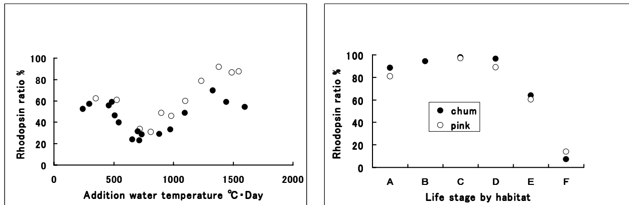
Fig. 3. Composition changes in retinal pigments in the hatchery (left view) and after release (right view). A—Japan coast after release, B—migrating north (maybe Honshu origin), C—in the Sea of Okhotsk before winter, D—during feeding or homing migration (caught by drift gillnet in the North Pacific Ocean), E—during homing migration (caught by set net), F—in river before spawning.
