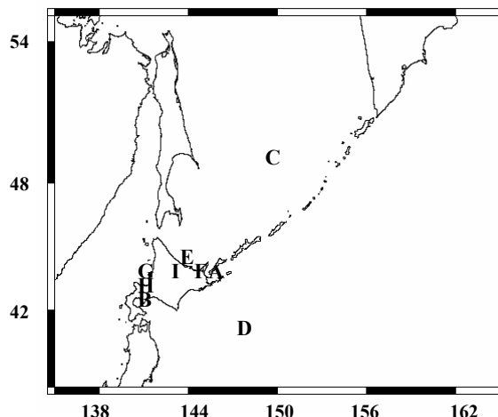
Fig. 1. Research area for the composition of visual pigments. A—offshore Shibetsu, B—offshore Shiraoui, C—Sea of Okhotsk, D—North Pacific Ocean, E—Tokoro R., F—Shari R. and set net, G—Atsuta, H, Chitose, I—Kitami.
