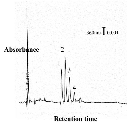
Fig. 2. Example of the chromatogram of a hatchery chum salmon just before release. 1—11-cis-retinaloxime, 2—11-cis-3-dehydroretinaloxime, 3—all-trans-retinaloxime, 4—all-trans-3-dehydroretinaloxime.
